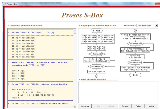
Gambar 2. Form Proses S-Box
